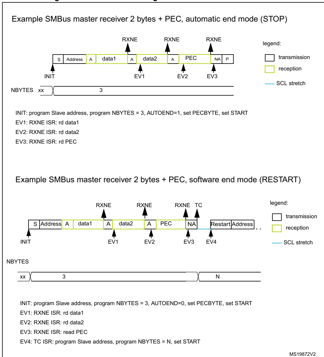
Figure 270. Bus transfer diagrams for SMBus master receiver
