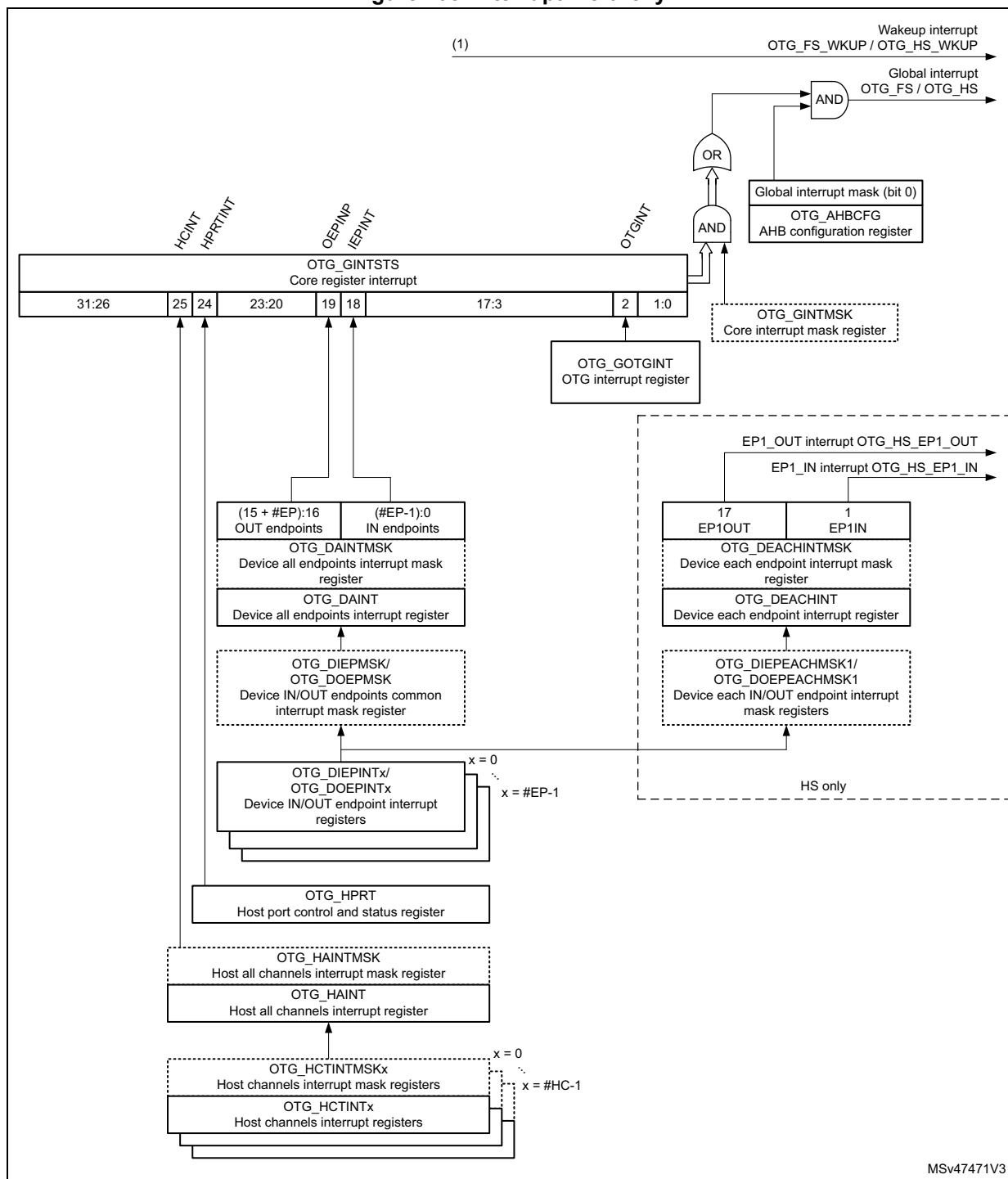
Figure 408. Interrupt hierarchy
