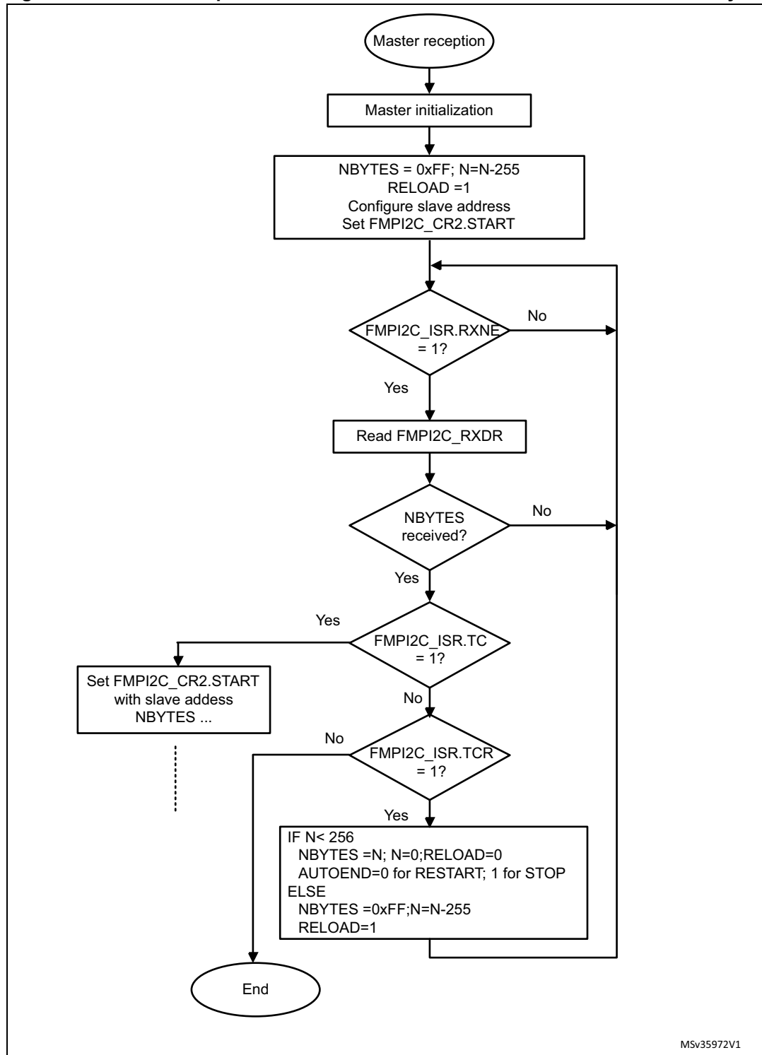
Figure 262. Transfer sequence flowchart for FMPI2C master receiver for N > 255 bytes
