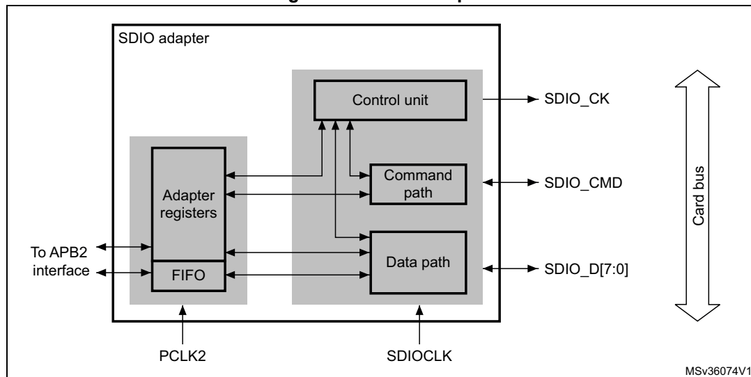
Figure 375. SDIO adapter
