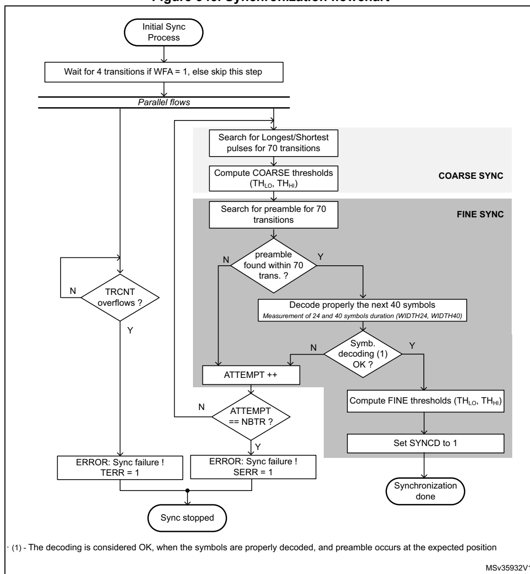
Figure 345. Synchronization flowchart
