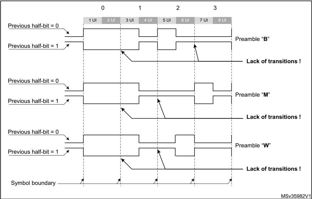
Figure 340. S/PDIF Preambles
