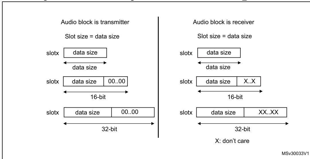
Figure 357. Slot size configuration with FBOFF = 0 in SAI_xSLOTR
