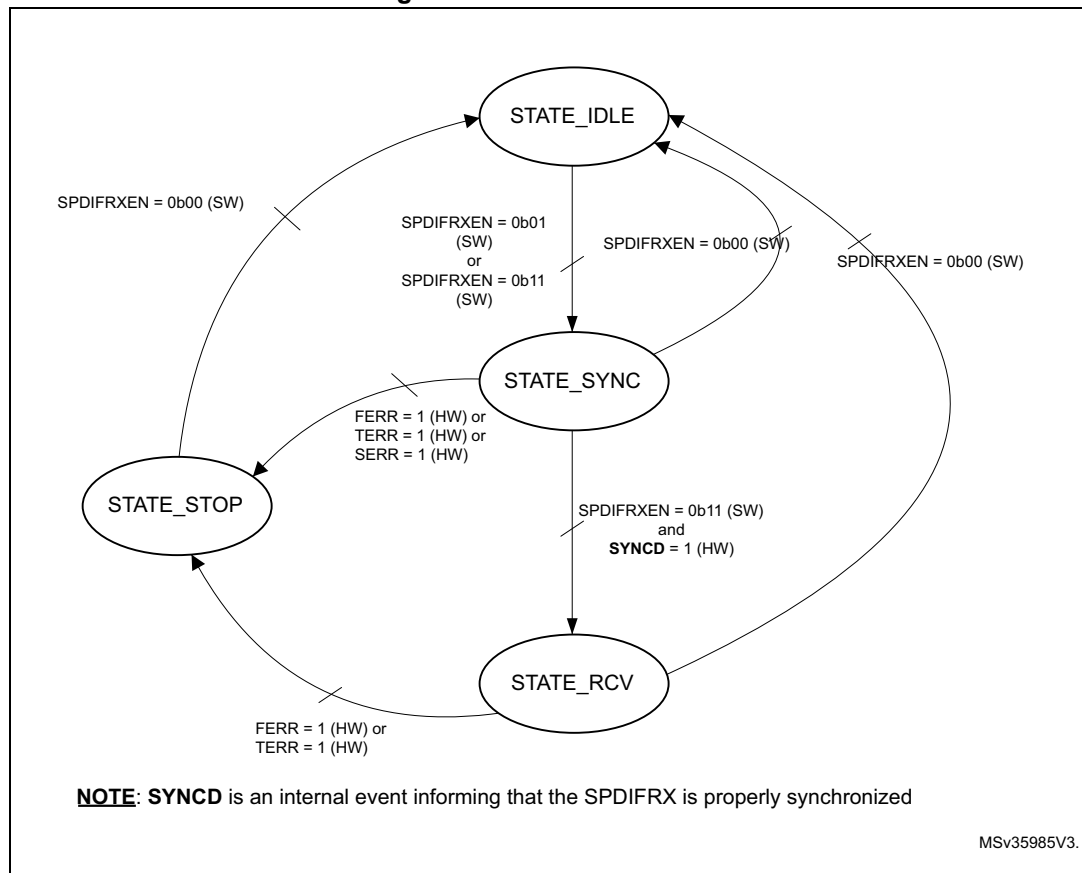
Figure 347. SPDIFRX States
