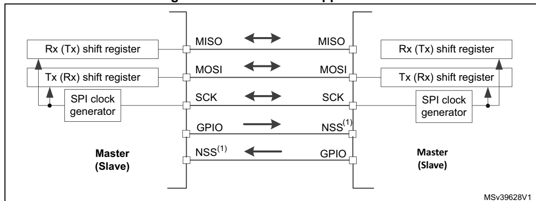
Figure 308. Multi-master application
