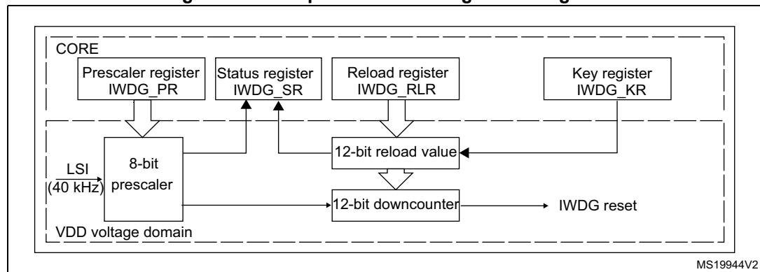
Figure 237. Independent watchdog block diagram
